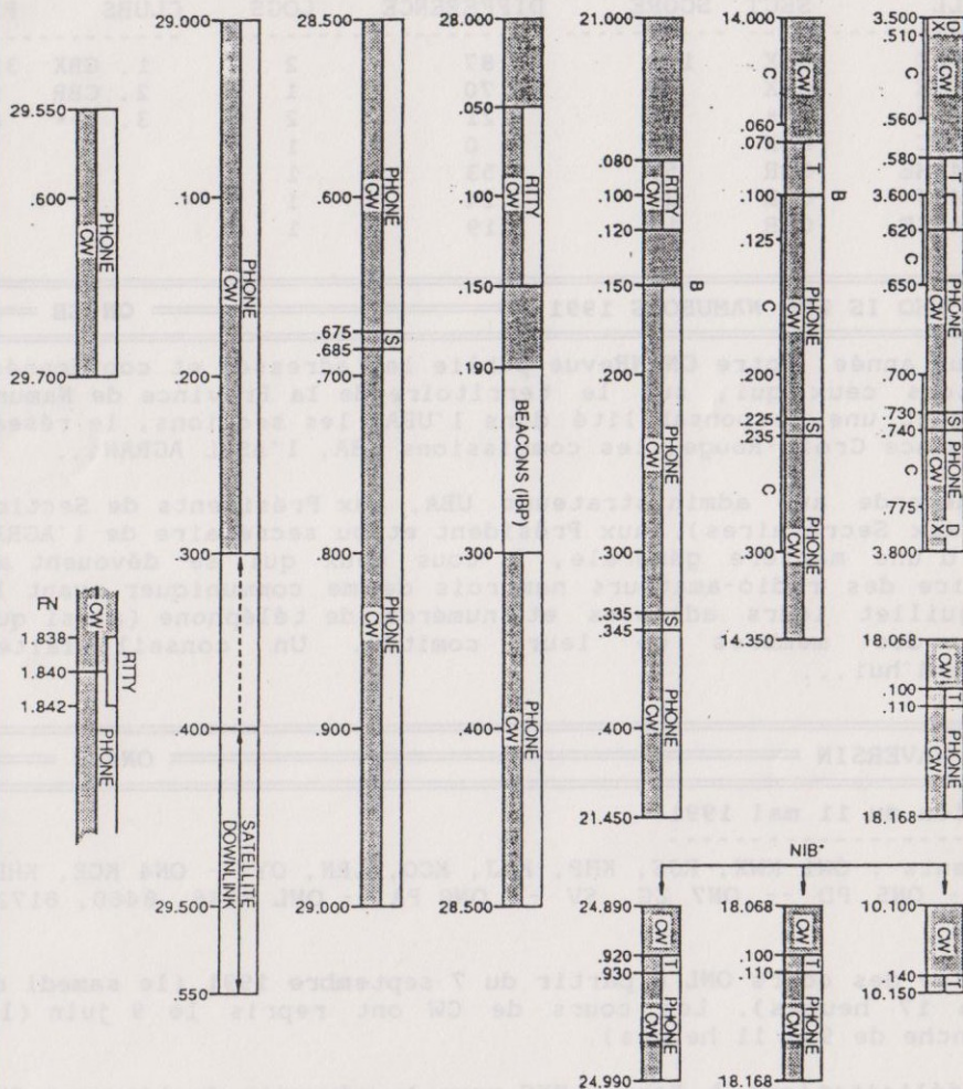
IARU Region I Band Plan (Frequencies in kHz)
